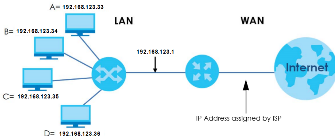
Figure 50 Multiple Servers Behind NAT Example
