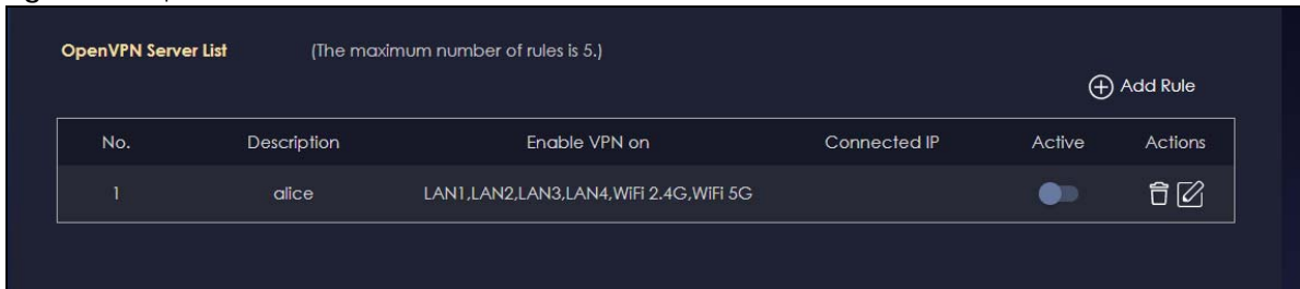
Figure 35 OpenVPN Client
