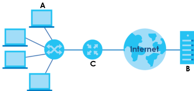
Figure 54 Port Trigger Process: Example
